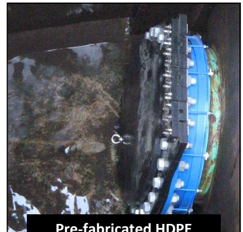
Pre-fabricated HDPE tidal flap valve
