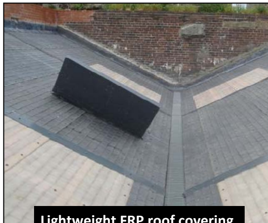
Lightweight FRP roof covering, Conwy Tower
